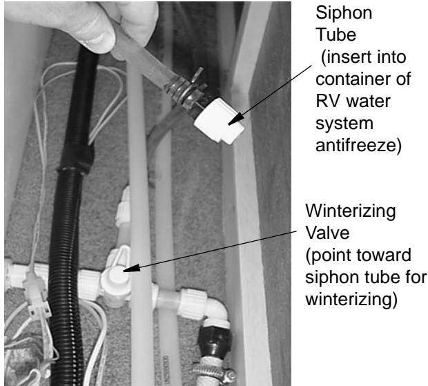
Winterization Valve
