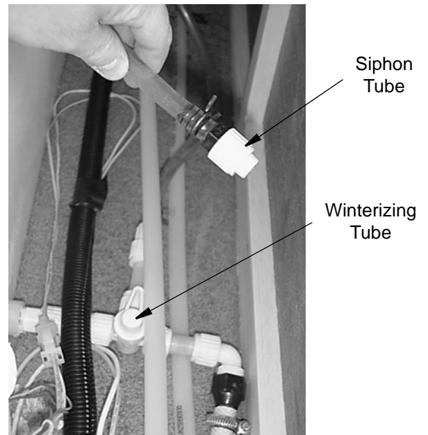
Winterization Valve beneath rear bed Models 30B & 33L shown
