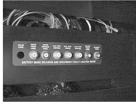
Chassis and House 12V Circuit Breakers behind cover panel in cargo compartment near entrance door
