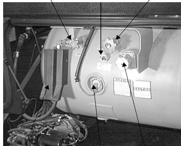
LP Gas Pressure Regulator Tank Gauge Tank Fill Valve
