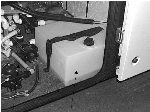
Water Pump RV Water System Antifreeze Reservoir
