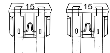
GOOD FUSE BAD FUSE
