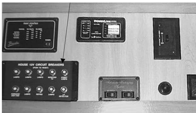
House 12-Volt Circuit Breaker Panel
