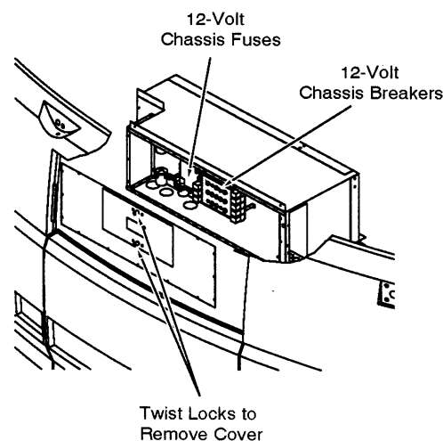
Automotive Fuse/Breaker Panel (Behind "Hood" Panel)
