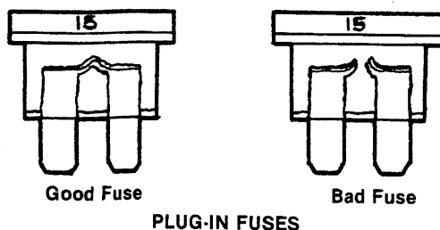
PLUG-IN FUSES
