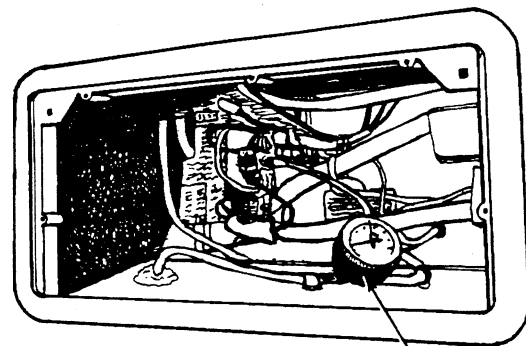
Leak Gauge
