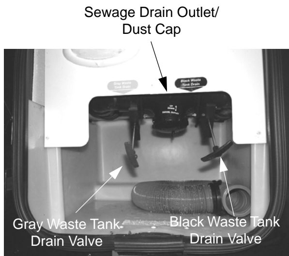
Holding Tank Drain Valves (Located in holding tank compartment) -Typical View
