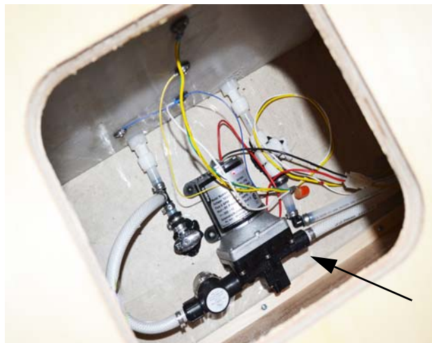
Water Pump (Located beneath bed - lift mattress to expose access hole) *Models 22R, 25B, 31G, and 31K
