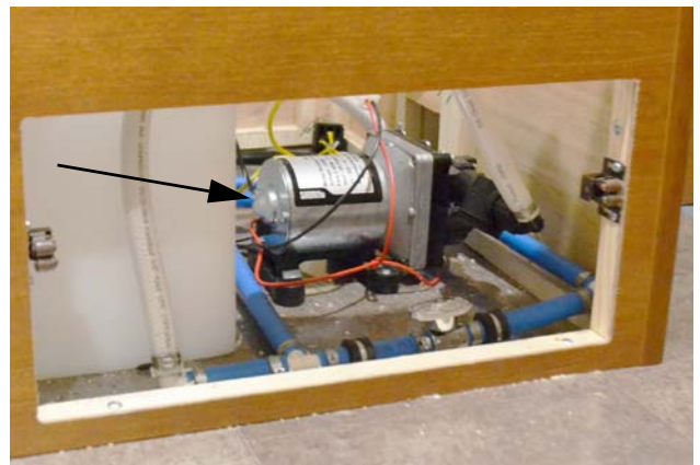
Water Pump (Located beneath bed - remove panel at foot of bed to access) *Model 31D
