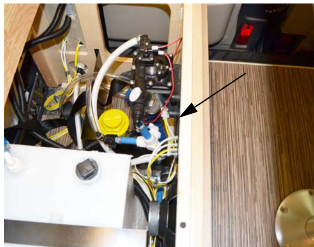
Winterization Valve 2 (Located beneath passenger side dinette seat)
