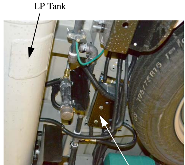
Pressure Regulator
