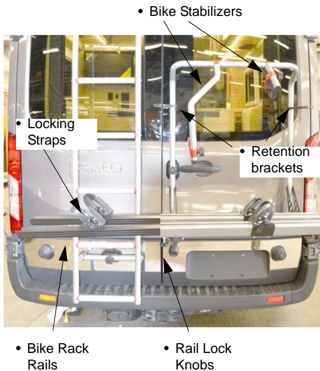
Bike Rack (shown in down position)
