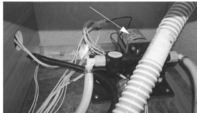
Water Pump (Located beneath step cover on side of bed. Extend backwall slideout to access.) -Model 24G shown
