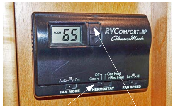
Thermostat Switch • Move to Heat or Gas position for furnace operation
