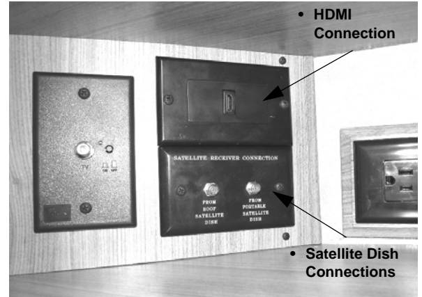
Interior Satellite Dish and HDMI Connections (Located near entertainment center cabinet) -Typical installation shown
