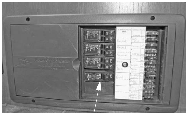
120-Volt House Circuit Breakers -Typical View
