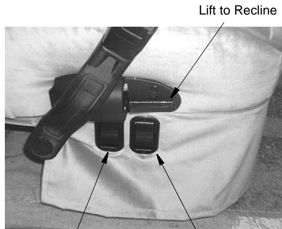
Lift to Swivel Lift to Slide Driver Seat - Aisle Side
