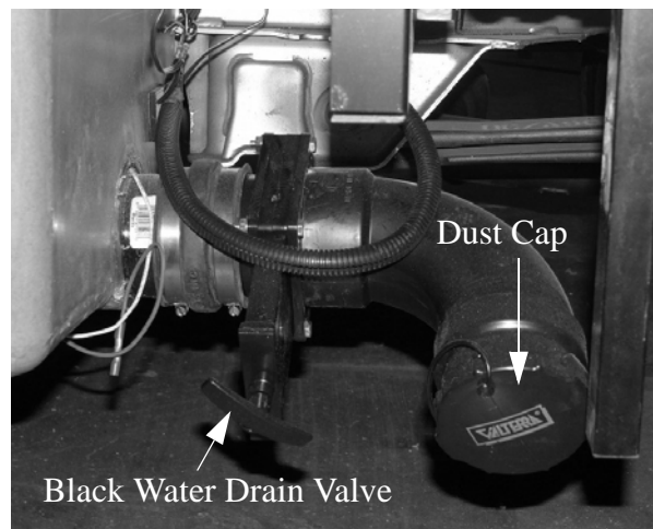
Black Water Sewage Drain Outlet (Located ahead of the driver rear wheel)
