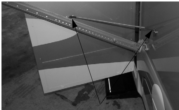
Insert ends of door prop into loop brackets on sidewall and door to provide adequate door clearance and avoid contact with awning arm.
