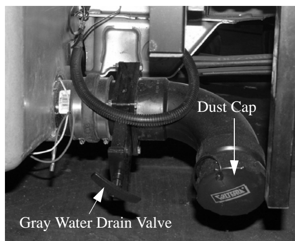
Gray Water Sewage Drain Outlet (Located behind the driver rear wheel)
